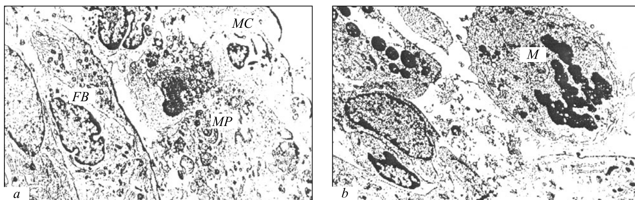
Fig. 3. The ultrastructural organization of the capsule and the subcapsular zone of spleen explant of 3-day-old rat: electron microscopy. Magnification: a ) \times 8200 , b ) \times 8750 . MC, mesothelial cells; MP, macrophages; FB, fibroblasts; M, mitosis.
